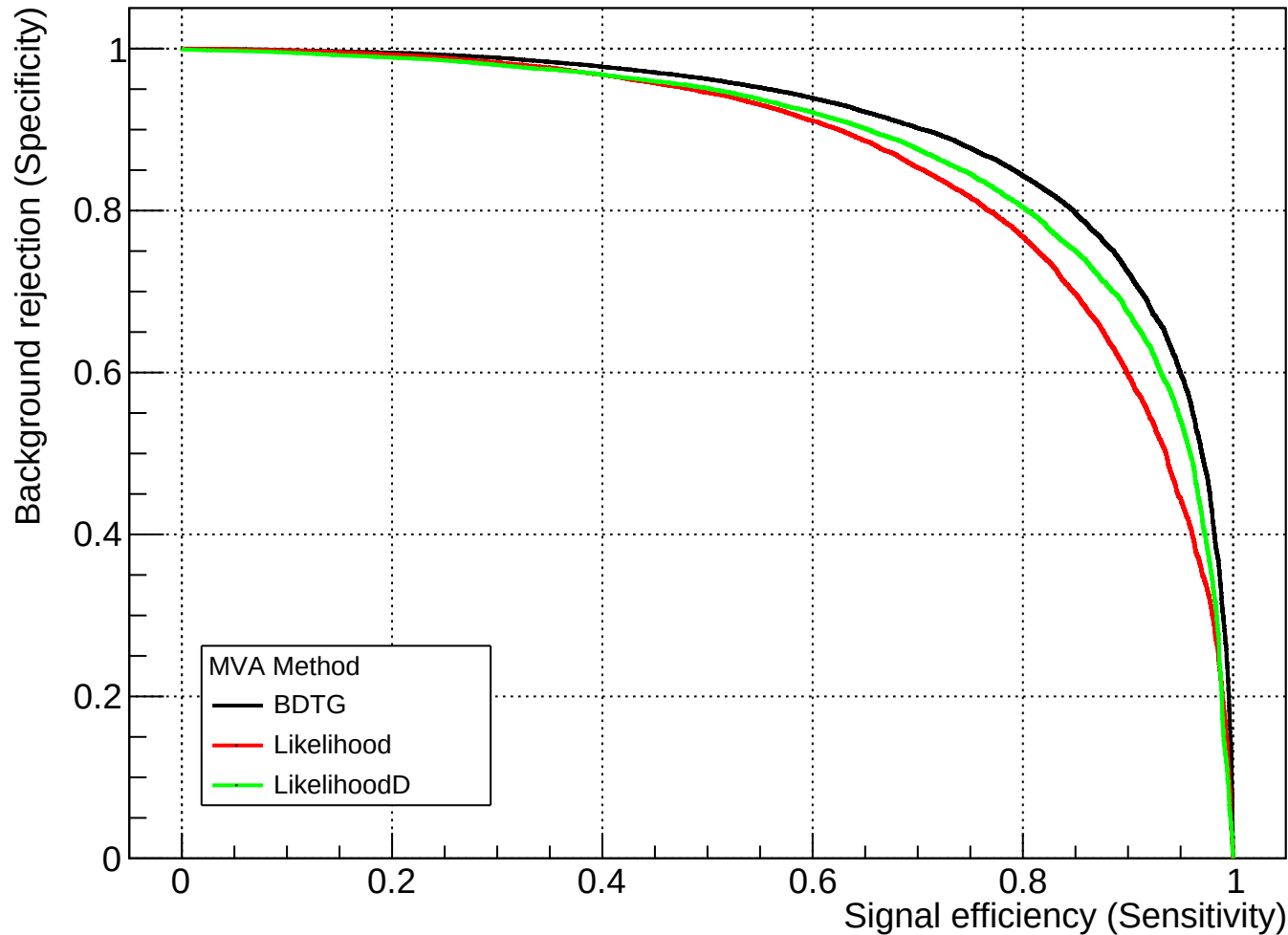
Signal efficiency vs. Background rejection
