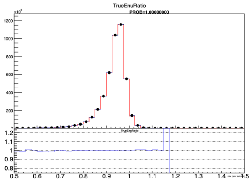
Minerva_KSprob_results/h__QElike__qelikenot__TrueEnuRatio__selected_truth_CV_WithErr
