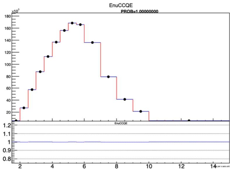
Minerva_KSprob_results/h_QElike_data_EnuCCQE_reconstructed_CV_WithErr
