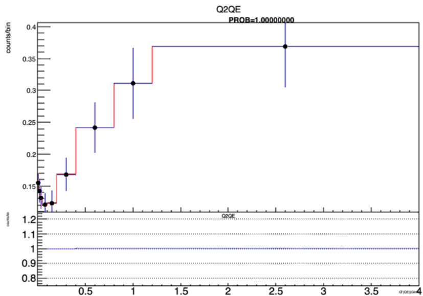
Minerva_KSprob_results/h_QElike_Q2QE_bkgfraction_CV_WithErr
