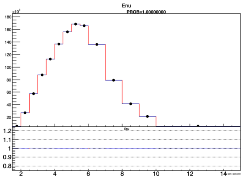
Minerva_KSprob_results/h__QElike__data__Enu__reconstructed_CV_WithErr
