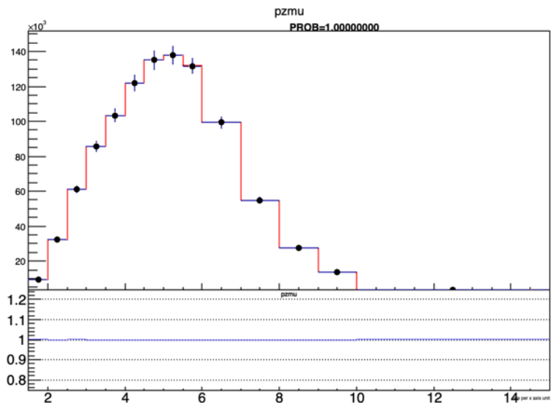
Minerva_KSprob_results/h_QElike_pzmu_bkgsb_CV_WithErr
