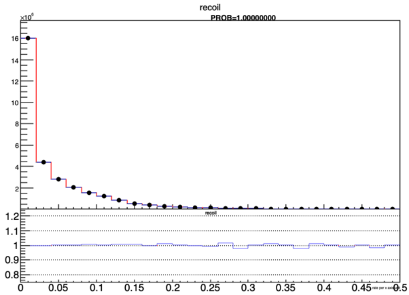
Minerva_KSprob_results/h_QElike_recoil_bkgsb_CV_WithErr
