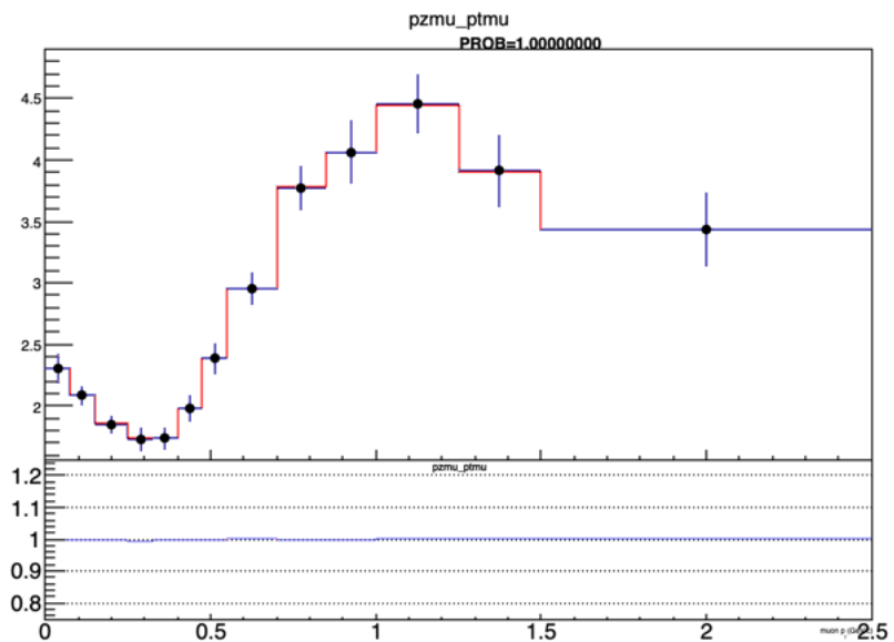
Minerva_KSprob_results/h2D_QElike_pzmu_ptmu_bkgfraction_CV_WithErr_py
