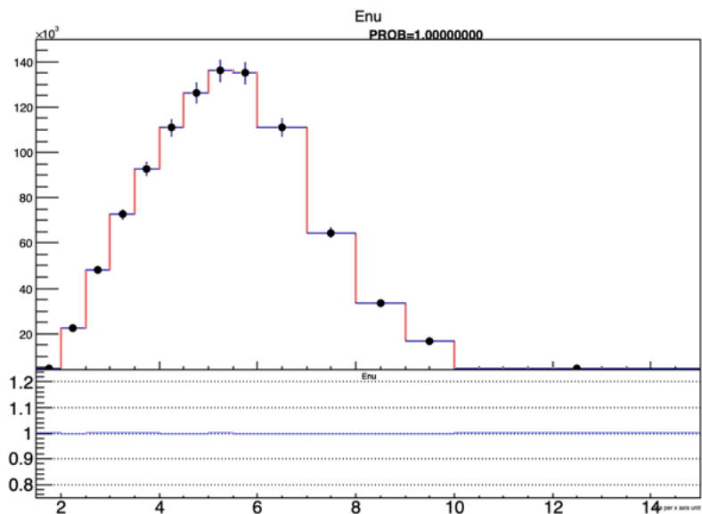
Minerva_KSprob_results/h_QElike_Eneu_bkgsb_CV_WithErr
